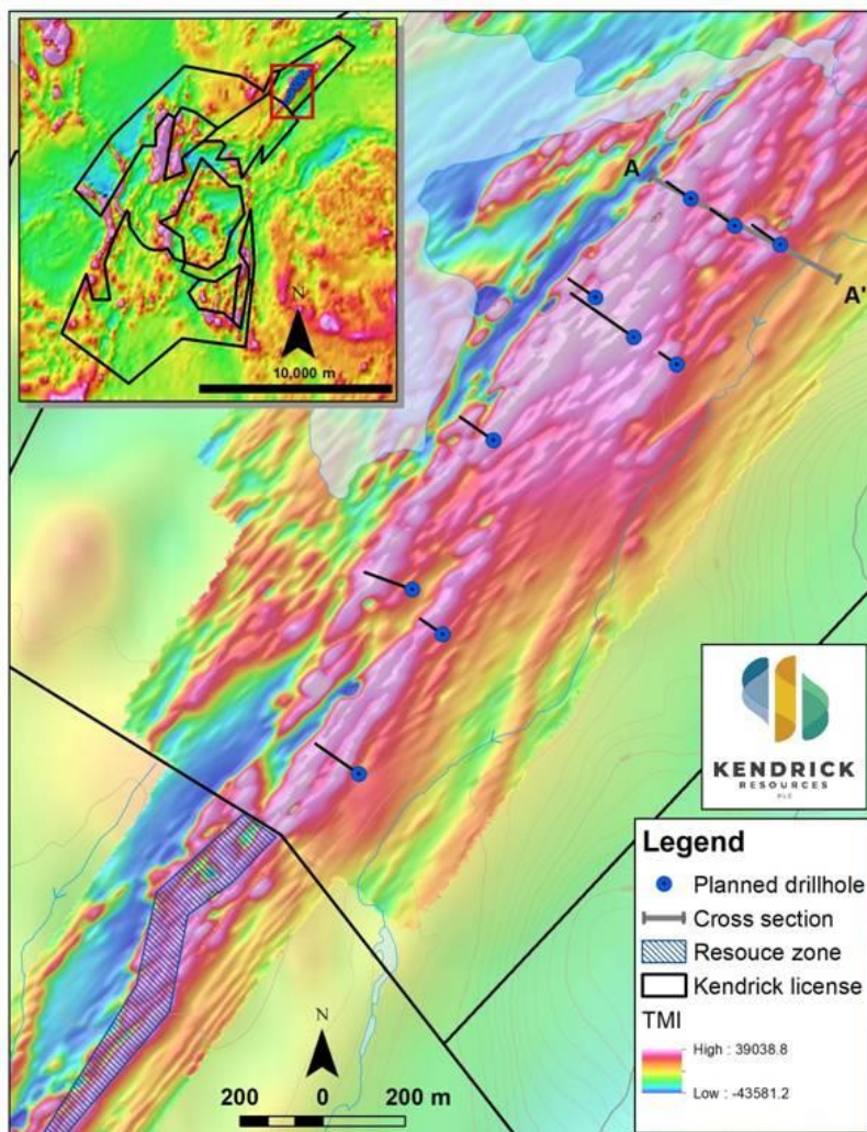
Magnetic map showing JORC resource and planned drilling (Source: www.kendrickresources.com )
