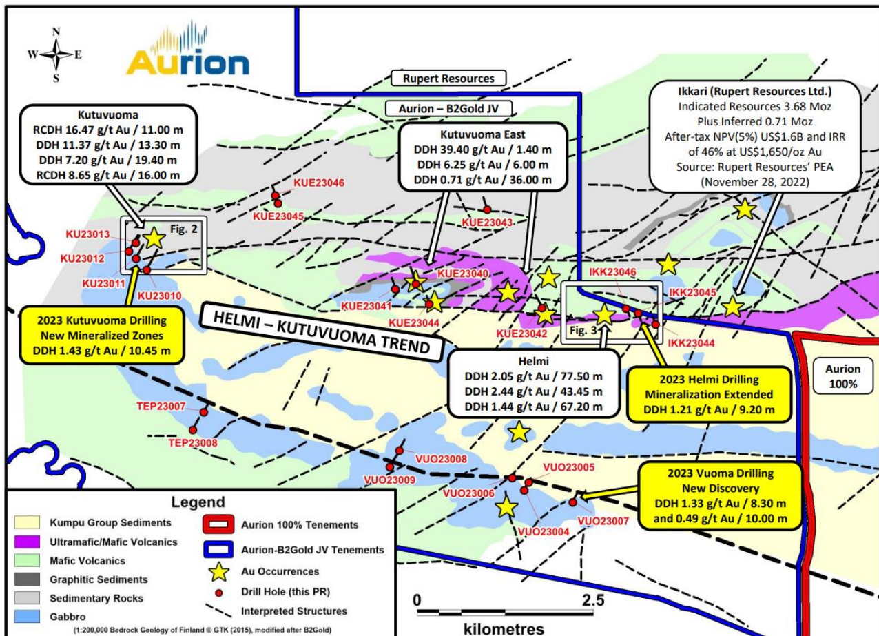
Exploration map over the Helmi-Kutuvuoma trend (Source: www.aurionresources.com )
