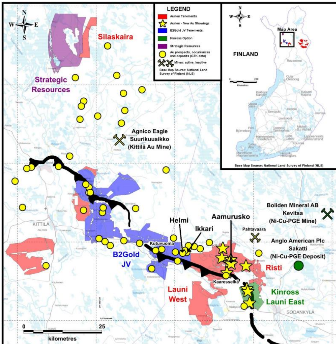
Aurion Resources' land tenements and interest in the CLGB (Source: www.aurionresources.com )
