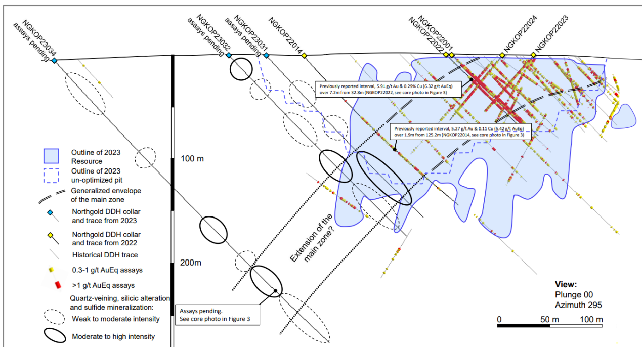
Cross section looking W-NW showing the 2023 Kopsa resource, un-optimized pit outlines, and drilling data (Source: www.northgoldab.com )
