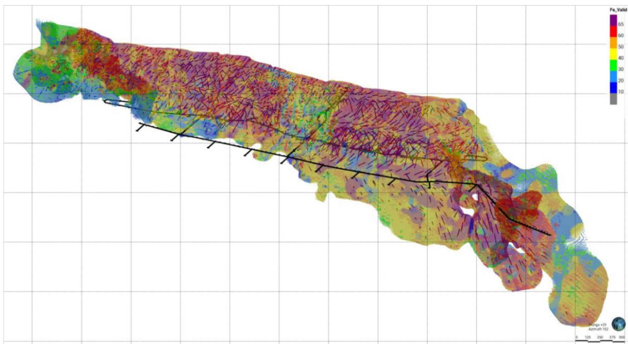
Kiruna Mineral Resource Model Coloured by Fe%
