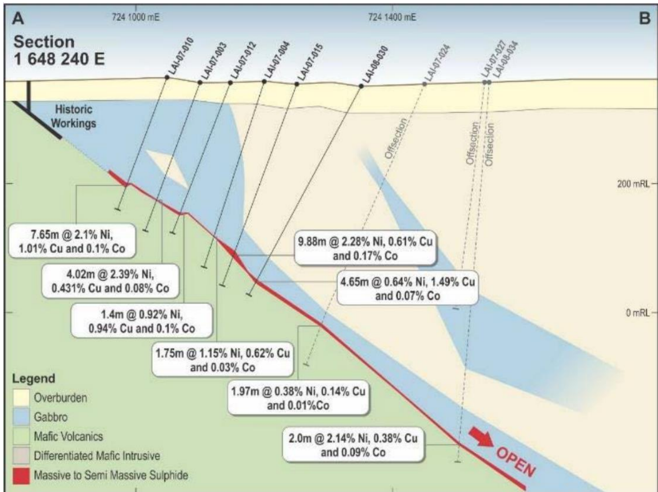
North-south section through Lainejaur (Source: www.bayrockresources.com)
