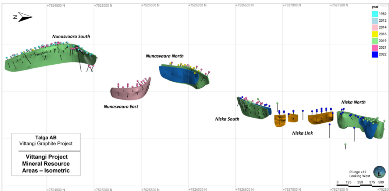
Vittangi Mineral Resource Domains (Source: www.talgagroup.com )
